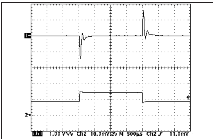
Figure 5: Output voltage response to step-change in load current (50% -75% -50% of I out (max); dI/dt = 0.1 A/μs). Load cap: 1 μF ceramic cap. Ch 1: V out , Ch 2: I out (5 A/div).
