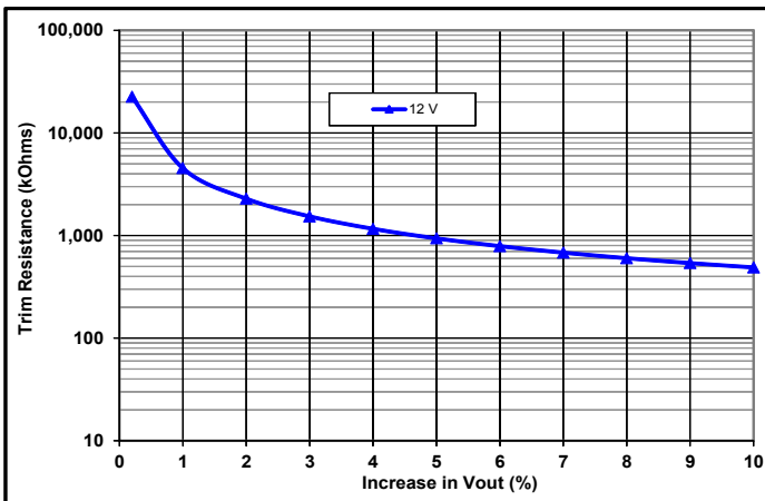
Common Figure 3: Trim graph for trim-up 12 V output.
