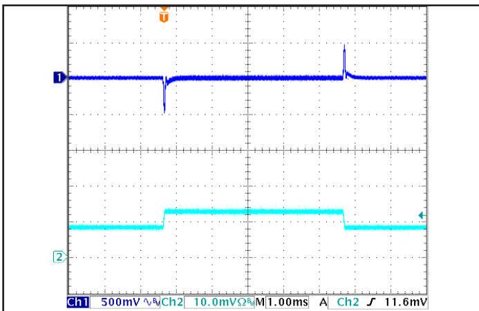
Figure 5: Output voltage response to step-change in load current (50% -75% -50% of I out (max); dI/dt = 0.1 A/μs). Load cap: 15 μF tantalum cap and 1 μF ceramic cap. Ch 1: V out , Ch 2: I out (10 A/div).
